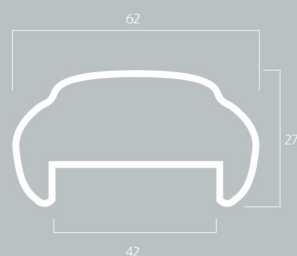
MT8-15/10=Kg/ml 1,87
