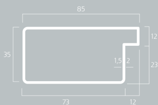
2D Kg/m 2,78
